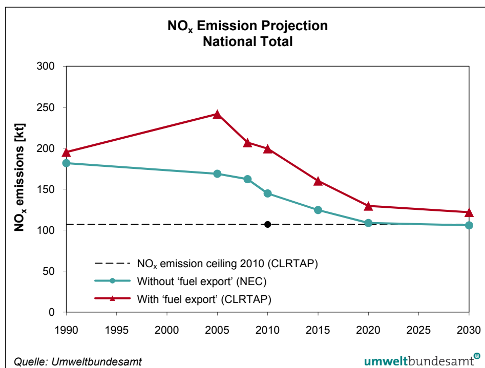
Figure 1: Historical (1990, 2005, 2008) and projected emissions (2010–2030) of NO x in comparison to the national emission ceiling (2010).
