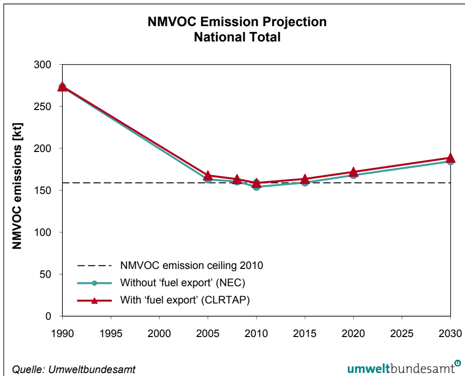
Figure 3: Historical (1990, 2005, 2008) and projected emissions (2010–2030) of NMVOC in comparison to the national emissions ceiling (2010).
