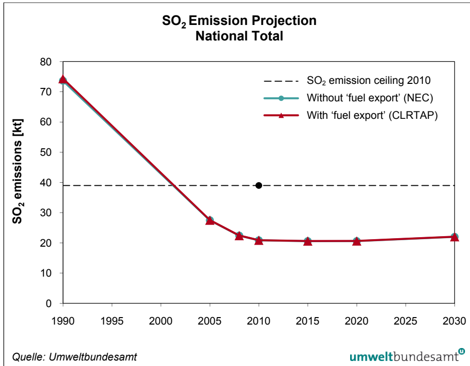
Figure 2: Historical (1990, 2005, 2008) and projected emissions (2010–2030) of SO 2 in comparison to the national emissions ceiling (2010).
