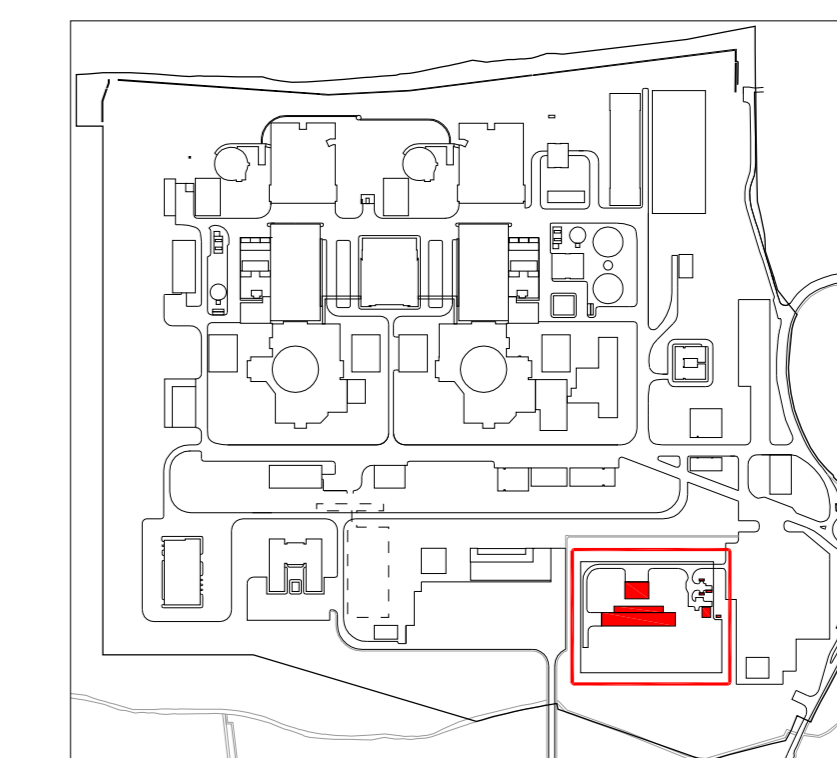
Hinkley Point C Site Key Plan - NTS
