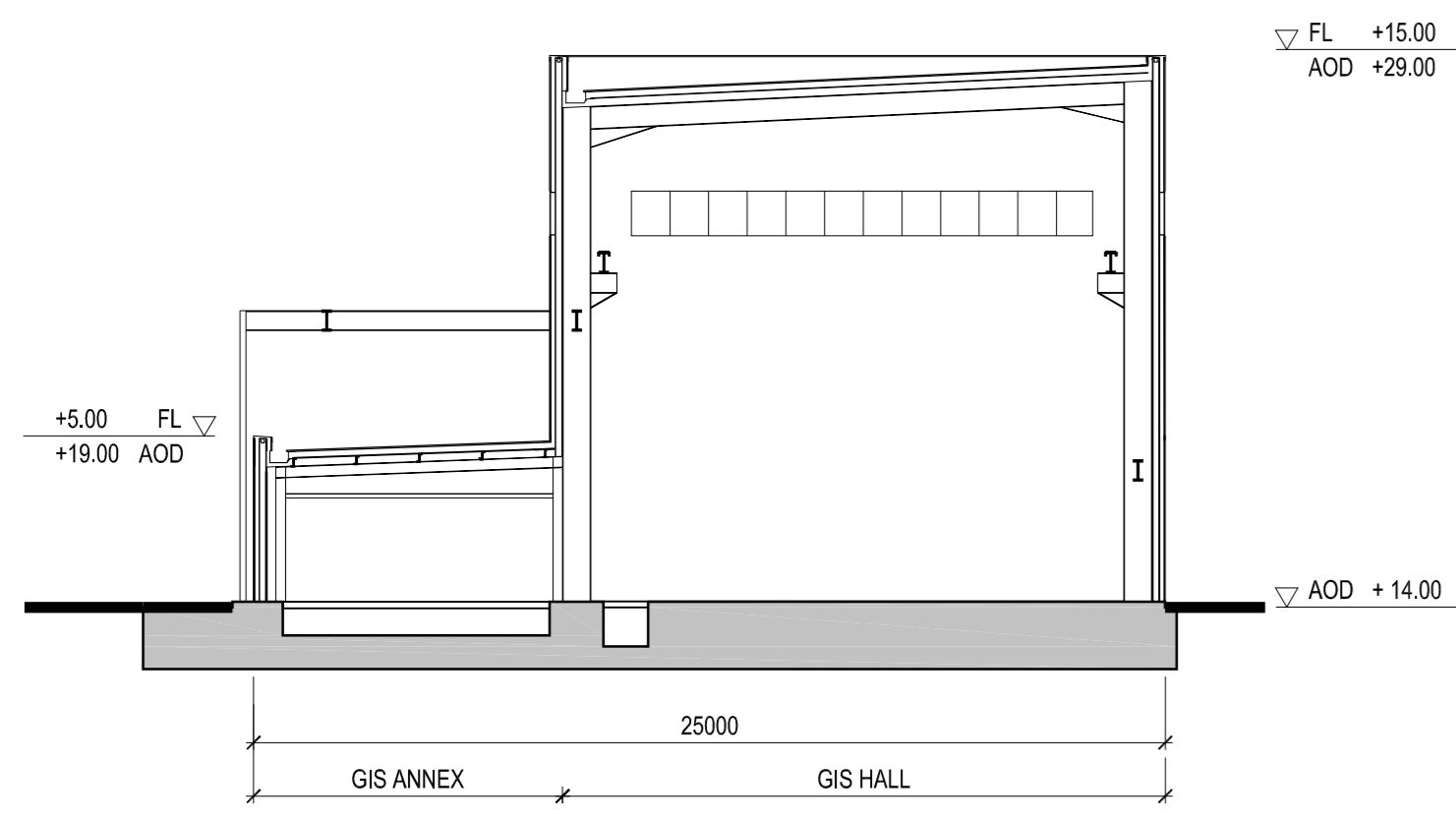
1 SECTION AA SCALE 1:200
