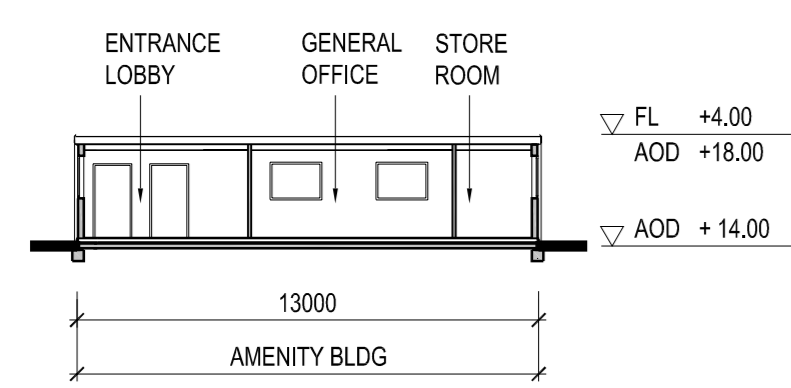
4 SECTION D/D SCALE 1:200
